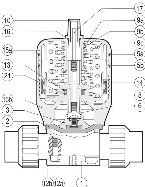
Normally Closed (NC)
